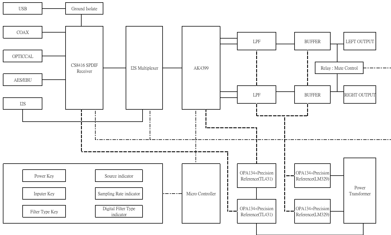
LOTUS DAC1 Block Diagram
